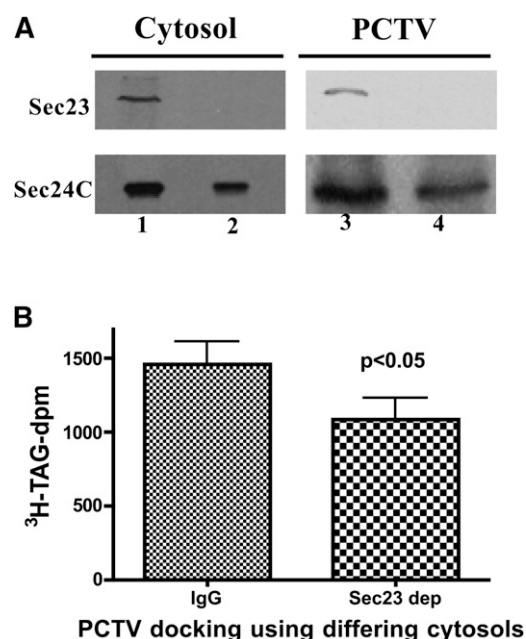
Fig. 2. The effect of Sec23 depletion from the cytosol and ER on PCTV docking with Golgi membranes. A: Sec 23 was immunodepleted from native rat cytosol using specific antibodies. 40 \mu g of cytosolic protein was separated by SDS-PAGE and Sec23 or Sec24C identified by ECL. Cytosol was immunodepleted by IgG or anti-Sec 23 antibodies as indicated. PCTV were generated using IgG depleted or Sec23 immunodepleted cytosol and its proteins separated by SDS-PAGE. Sec23 or Sec24C was identified by immunoblot using anti-Sec23 or Sec24C antibodies as shown. B: PCTV (150 \mu g protein) were generated using IgG or Sec23 immunodepleted cytosol and were docked with Golgi membranes (300 \mu g protein). The 3 H-TAG-dpm associated with the Golgi was determined in each case (ordinate). The P value tests the differences between the means \pm 1 SEM, N = 4. ECL, enhanced chemiluminescence; ER, endoplasmic reticulum; PCTV, prechylomicron transport vesicle; TAG, triacylglycerol.
