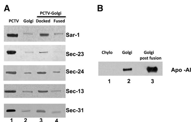
Fig. 1. The effect of docking and fusion of PCTV with Golgi membranes on COPII proteins and chylomicron acquisition of apoAI on fusion with the Golgi. A: Equal amounts of proteins (40 \mu\text{g} ) were separated by 12% SDS-PAGE, transblotted to nitrocellulose membranes, and the proteins detected by ECL using specific antibodies to the COPII proteins as indicated. The presence of the COPII proteins was detected in PCTV (lane 1), Golgi (lane 2), PCTV docked with the Golgi (lane 3), and PCTV fused with the Golgi (lane 4). Methods for docking and fusion of PCTV with the Golgi are described in "Materials and Methods." B: Chylomicrons isolated from PCTV (lane 1), Golgi prior to fusion with PCTV (lane 2), and Golgi after fusion with PCTV (lane 3) were obtained and their proteins separated by SDS-PAGE. After transblotting, apoAI was identified by ECL using specific antibodies. ECL, enhanced chemiluminescence; PCTV, prechylomicron transport vesicle.
