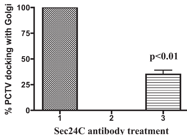
Fig. 6. Sec24C antibody treatment of PCTV blocks its docking with Golgi membranes. ^3 H-TAG loaded PCTV were generated using native cytosol and ER and docked with Golgi membranes. The ^3 H-dpm found associated with the Golgi under these conditions was set to 100% (bar 1). In bar 2, cytosol and ER immunodepleted of Sec24C was used to generate PCTV devoid of Sec24C that was then incubated in Sec24C depleted cytosol with Golgi membranes. The percentage of ^3 H-dpm found docked with the Golgi under these conditions as compared with when native PCTV was used is shown. In bar 3, PCTV formed using native cytosol and ER were treated with 20 \mu l of anti-Sec24C antibody at 4°C for 30 min and then incubated with native cytosol and Golgi in a docking assay. The percentage of ^3 H-TAG-dpm associated with the Golgi under these conditions as compared with the results obtained in bar 1 are shown. The P values test the difference between the means for bar 1 and bar 3. The data are the mean \pm SEM, N = 4. PCTV, prechylomicron transport vesicle; TAG, triacylglycerol.
