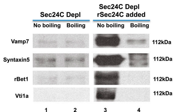
Fig. 5. The effect of Sec24C immuno-depletion on the formation of the PCTV-Golgi SNARE complex. PCTV were generated using Sec24C depleted cytosol and ER (Sec24C Depl, lanes 1 and 2) or PCTV generated in Sec24C depleted cytosol and ER followed by the incubation of the PCTV with rSec24C (29 \mu g) (Sec24C Depl, rSec24C added, lanes 3 and 4). The PCTV were then docked with the Golgi. Post docking, the Golgi membranes were isolated, solubilized in 2% Triton X-100, and the proteins immuno-precipitated using bead-bound anti-VAMP7 antibodies. The beads were not boiled or boiled in Laemmli's buffer as indicated. The proteins were separated by SDS-PAGE, transblotted, and the transblots probed using specific antibodies to the expected SNARE proteins (2). The blots shown are at 112 kDa, the Mr of the PCTV-Golgi SNARE complex (2). On boiling, the SNARE proteins disassociated from the complex and moved at their monomer Mr (data not shown). ER, endoplasmic reticulum; PCTV, prechylomicron transport vesicle.
