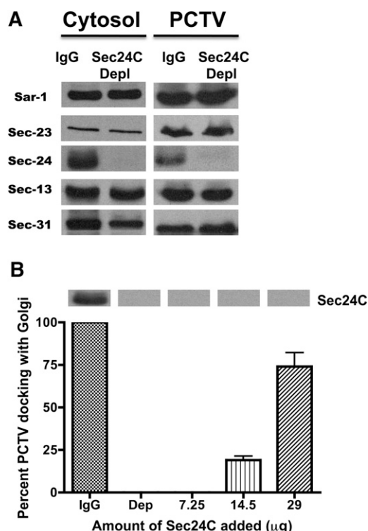
Fig. 3. Depletion of Sec24C from cytosol and ER impairs PCTV-Golgi docking. A: The effect of Sec24C immuno-depletion of cytosol on cytosolic COPII proteins. Cytosol: Rat intestinal cytosol was either immunodepleted with IgG (IgG) or anti-Sec24C antibodies (Sec24C Depl) as indicated and the cytosol probed for the COPII proteins using specific antibodies. 40 μg cytosolic protein was separated by SDS-PAGE and the COPII proteins identified using ECL after transblotting. The Sec23 band density of cytosol was quantitated using the Gel Doc XR Imaging System (BioRad). PCTV: PCTV (40 μg prot) formed using either IgG (IgG) or Sec24C immunodepleted (Sec24C Depl) cytosol was immunoblotted for the COPII proteins including Sec24C after separation by SDS-PAGE and the proteins identified by ECL after transblotting. B: The effect of Sec24C immunodepleted cytosol on PCTV docking with the Golgi and the effect on docking activity of adding recombinant Sec24C to Sec24C depleted cytosol. PCTV were generated in either IgG depleted (IgG) or Sec24C depleted rat intestinal cytosol to which either none (Dep) or the indicated amount of rSec24C had been added. The Sec24C status of the cytosols prior to the addition of rSec24C is shown above the graph in immunoblots. In each case, the ^3\text{H} -TAG loaded PCTV were docked with intestinal Golgi and the ^3\text{H} -TAG-dpm associated with the Golgi determined. The dpm (2946 ^3\text{H} -TAG-dpm) found for PCTV formed in IgG depleted cytosol was set to 100%. The data are the percentage of ^3\text{H} -TAG dpm associated with the Golgi by comparison to the dpm of IgG depleted cytosol. The data are the mean values \pm 1 SEM, N = 4. ECL, enhanced chemiluminescence; ER, endoplasmic reticulum; PCTV, prechylomicron transport vesicle; TAG, triacylglycerol.
