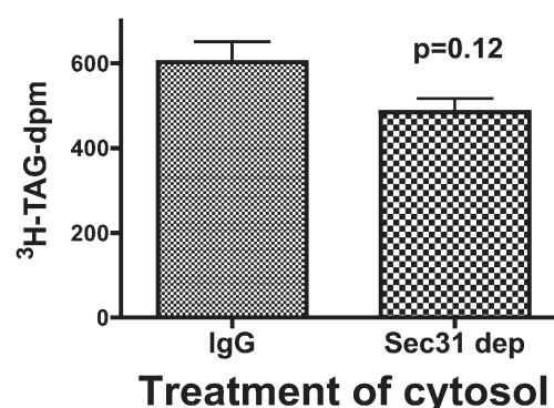
Fig. 4. The effect of Sec31 immunodepletion on PCTV docking with intestinal Golgi. Cytosol immunodepleted of Sec31 (data not shown) using specific anti-Sec31 antibodies or IgG was used to generate PCTV. PCTV (150 μg protein) formed using these cytosols were docked with intestinal Golgi (300 μg protein) as described in "Materials and Methods." After incubation, the number of ^3\text{H} -TAG-dpm associated with the Golgi was determined. IgG indicates PCTV formed in IgG depleted cytosol and Sec31 dep indicates Sec31 depleted cytosol. The data are the means \pm 1 SEM, N = 4. PCTV, prechylomicron transport vesicle; TAG, triacylglycerol.
